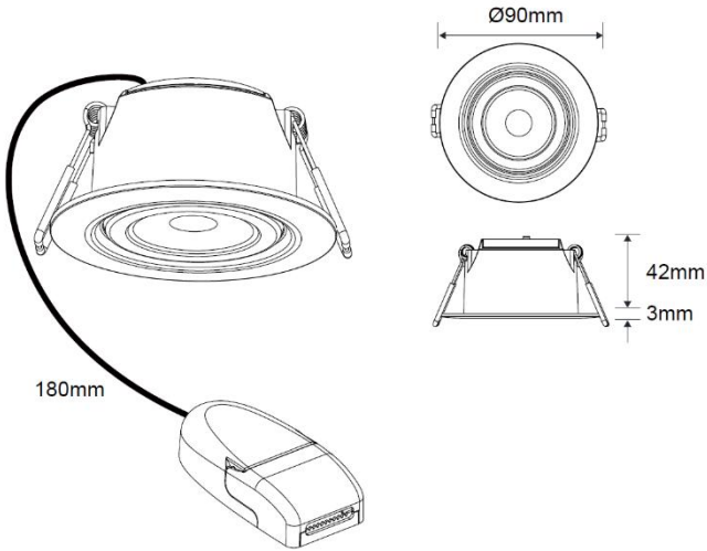
Dimension Diagram
